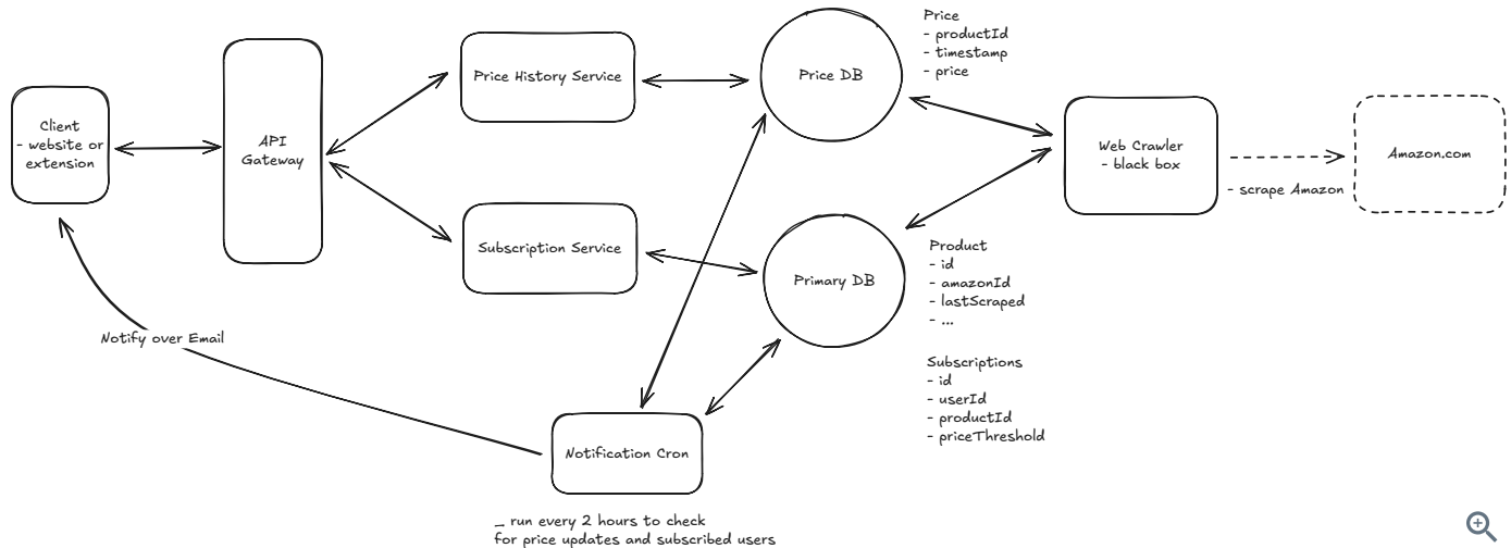
CamelCamelCamel High Level Design - Subscriptions
