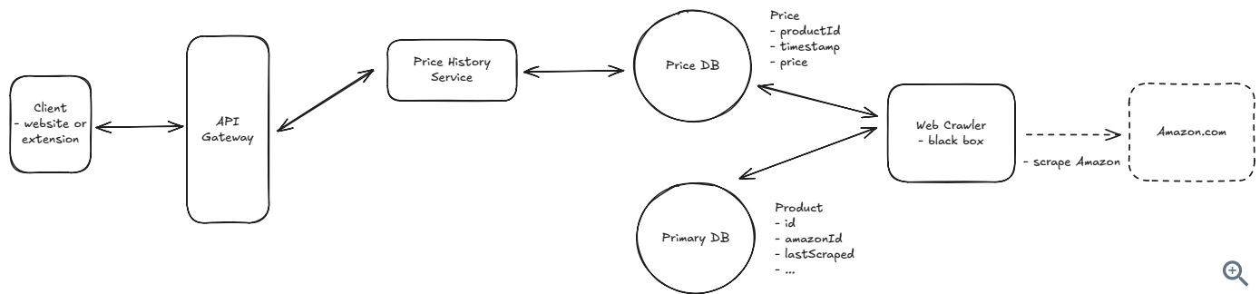
CamelCamelCamel High Level Design - Price History
